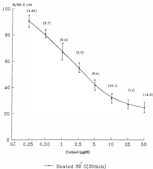
Fig. 4. Standard curve of cortisol by enzyme immunoassay in serum. Results of ten experiments. Values in parentheses = CV, Bars=SD.
