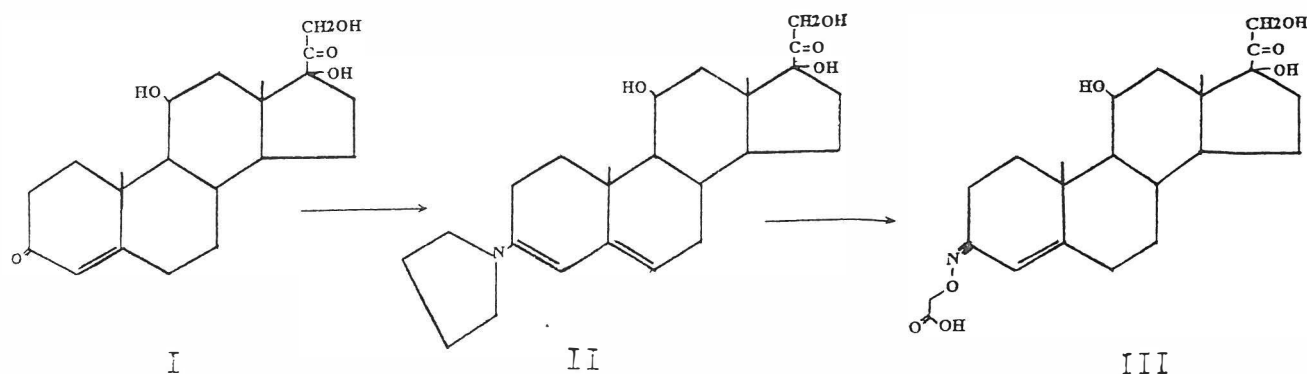
Fig. 1. Preparation of carboxymethyloxime derivative of cortisol.
