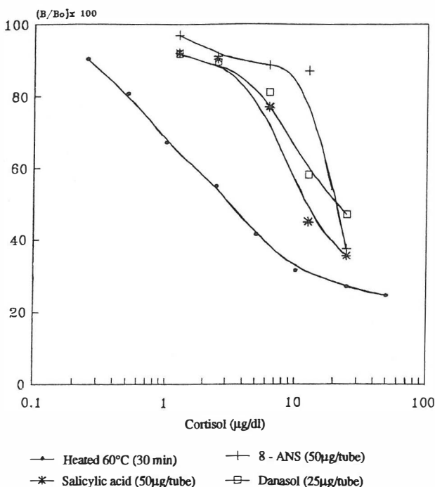
Fig. 5. Comparison of standard curves of cortisol using heat denaturation and blockers. Heat denaturation procedure was selected.
