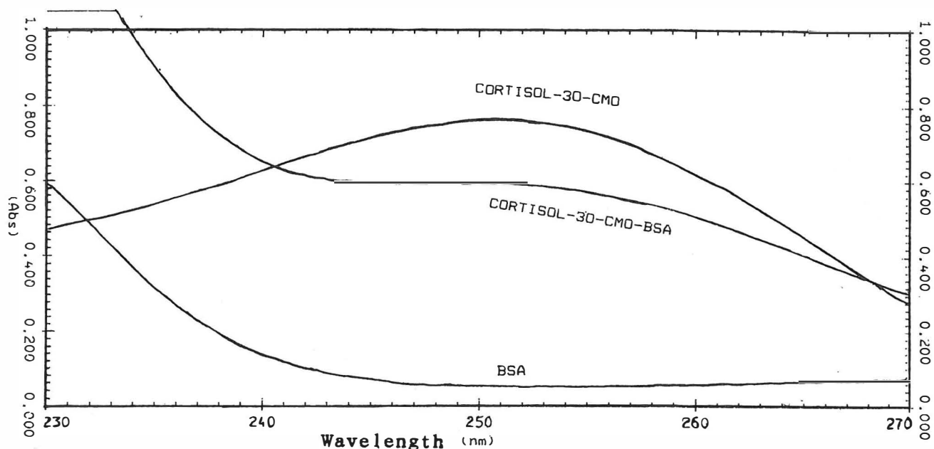
Fig. 2. Absorption spectra of BSA, cortisol derivative and its BSA conjugate.
