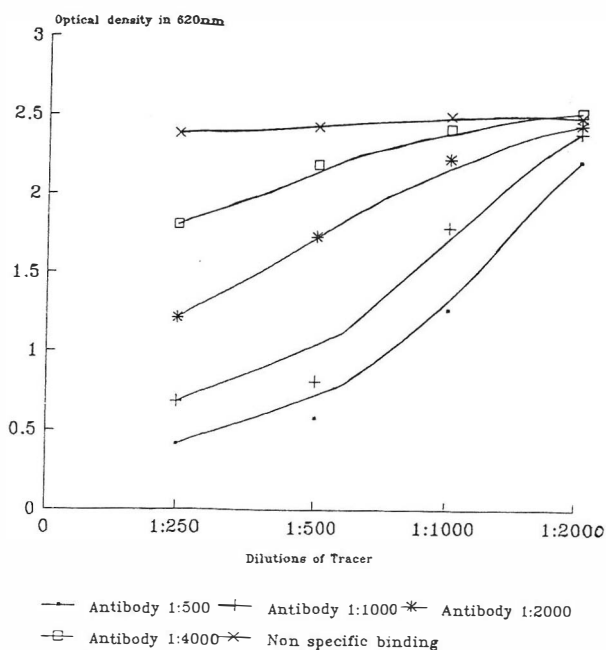
Fig. 3. Checker board titration of antibody raised after 75 days. Optimum dilution of Ab is 1/1000, optimum dilution of tracer is 1/500.
