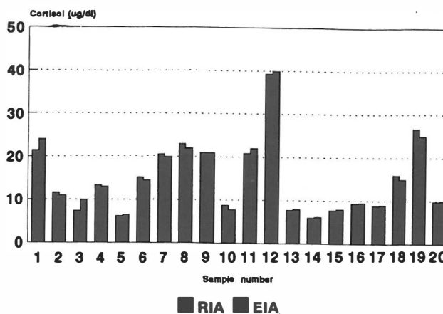
Fig. 6. Comparison of results obtained for 20 samples assayed by RIA and EIA.
