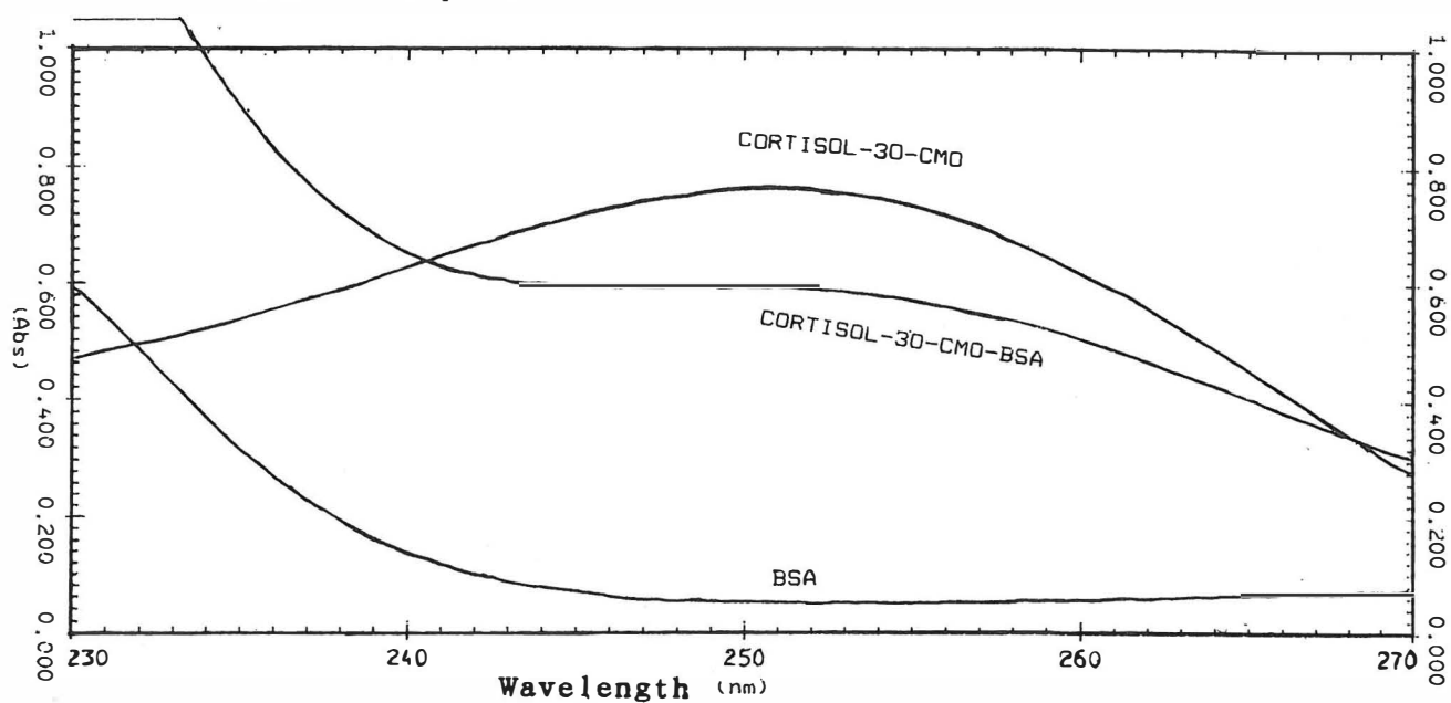
Fig. 2. Absorption spectra of BSA, cortisol derivative and its BSA conjugate.
