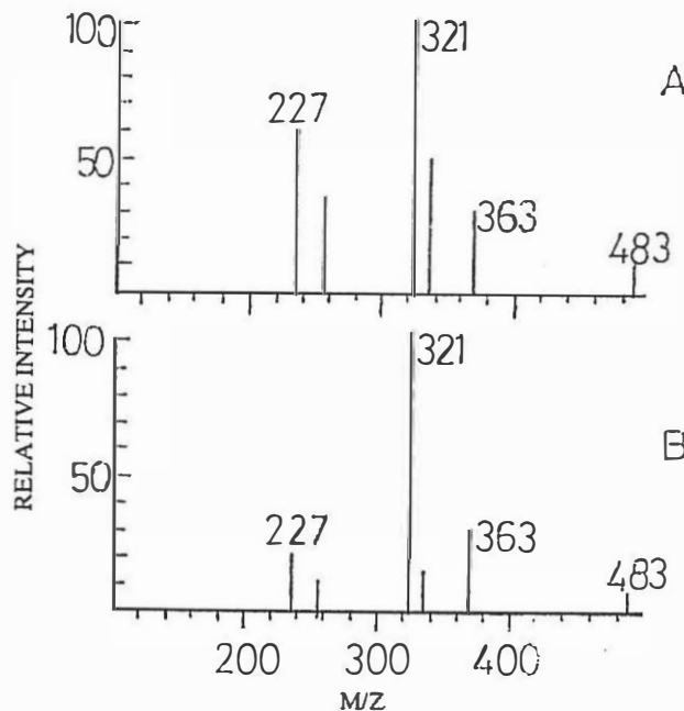
Fig.4. Electron ionisation mass spectra of: A. Methylated and acetylated urinary butobarbitone N-glucoside B. Synthetic butobarbitone- N- methyl- N'- (2, 3, 4, 6- tetra- O- acetyl- \beta - D- glucopyranoside.
