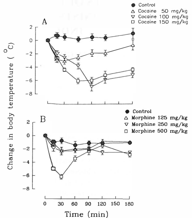
Fig. 1. Morphine and cocaine effects on body temperature. (A) Mice were treated subcutaneously with saline control (●, 10 mg/mL) and different doses of cocaine (Δ, 50; ▽, 100; □, 150 mg/kg). (B) Mice were treated subcutaneously with saline control (●, 10 mg/mL) and different doses of morphine (Δ, 125; ▽, 250; □, 500 mg/kg). Body temperature was determined at 15, 30, 60, 90 and 180 min after drug administration. Each point is the mean \pm SEM of 9 animals.
