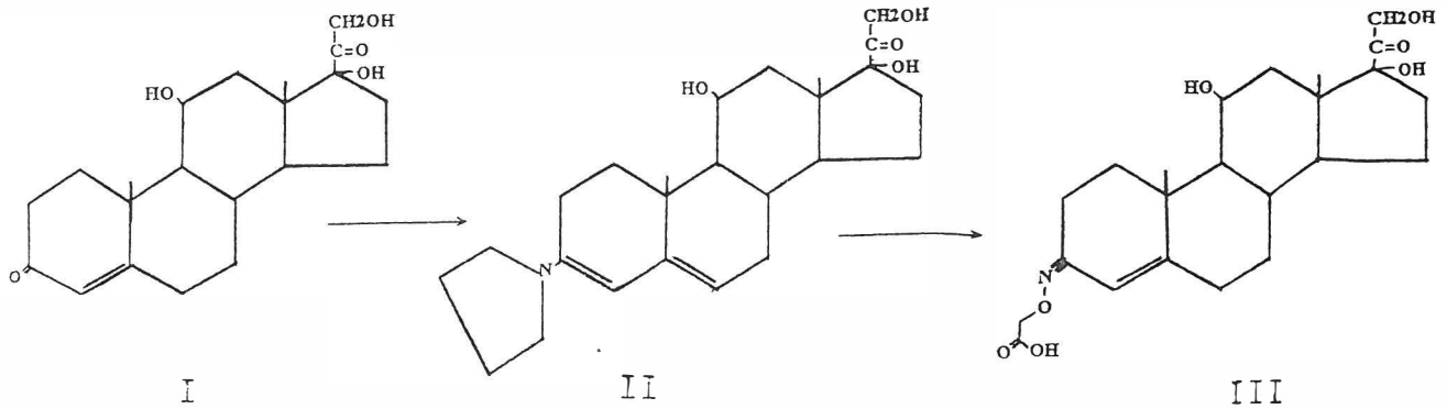
Fig. 1. Preparation of carboxymethyloxime derivative of cortisol.
