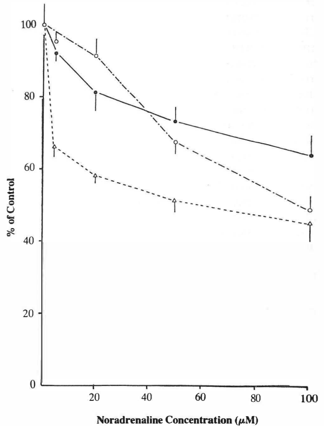
Fig. 2. Effect of reduced pterin cofactor on inhibition of dopamine synthesis by noradrenaline in striatal synaptosomes.
