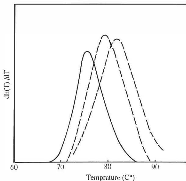
Fig. 5. Thermal denaturation profile of the interaction of DNA with sulfur mustard at 10 and 50 \mu\text{g}/\text{mL} concentrations. Derivative of the points obtained from four separate experiments is shown.
