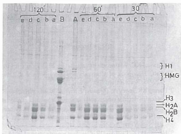
Fig. 3. SDS-polyacrylamide gel electrophoresis pattern of mustard treated and controls at 25°C. a-e of each experiment are zero to 50 µg/mL concentrations of sulfur mustard, respectively. A; standard calf thymus histones. B; standard nonhistone proteins (HMG).
