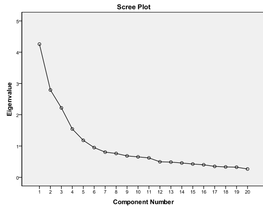
Fig. 1. Scree plot
