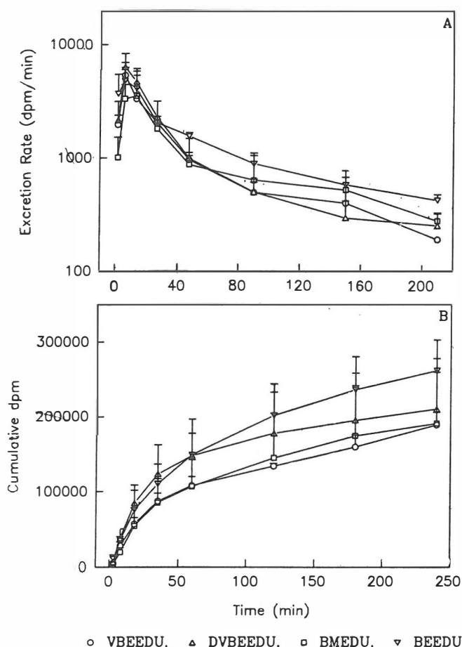
Fig. 3. Excretion rates (A) and cumulative excretion of radioactivity in bile samples (B) after injection of [4- 14 C]-(5S, 6S)-BMEDU, [4- 14 C]-BEEDU, [4- 14 C]-VBEDU and [4- 14 C]-DVBEEDU into rats. Values are the means \pm SD (n=3).
