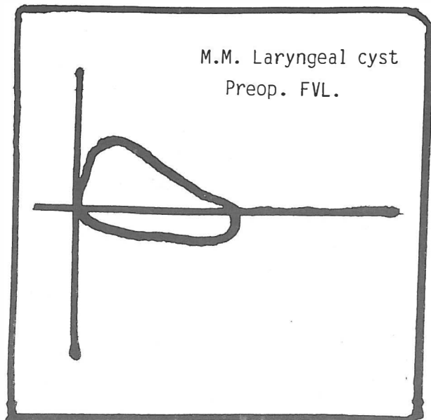
Fig. 5. Preoperative FVL.
