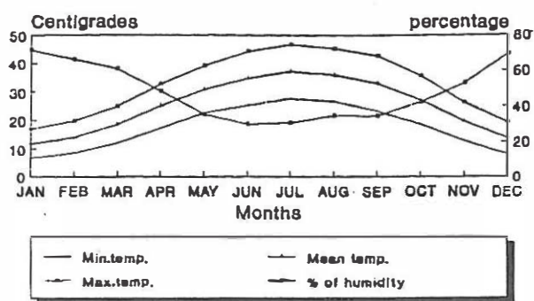
Fig. 4. Averages of temperature variations and humidity percentage of Ahwaz, capital of Khoozestan province (1980-1989).
