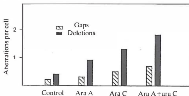
Fig.3. Frequencies of deletions and gaps induced by ara A (100 μmol/l) or ara C (100 μmol/l) alone or in combination in A-T cells exposed 4 h before fixation.
