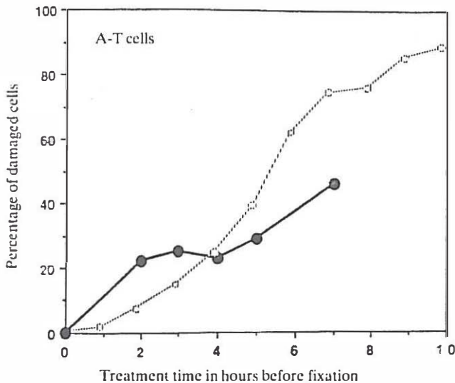
Fig.4. Percentage of damaged A-T cells following exposure to ara C (100 \mu mol/l) for various time intervals before fixation. Values for each point are subtracted from the number of damaged cells in the controls. The dotted line shows the percentage of labelled mitoses as a function of time before fixation in A-T cells.
