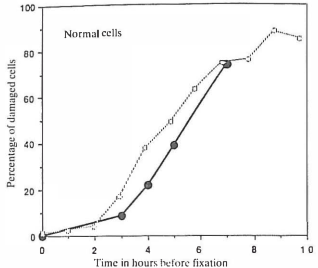
Fig.5. Frequency of damaged cells following exposure of normal cells to ara A (200 \mu mol/l) for various time intervals before fixation. Values for each point are subtracted from the number of damaged cells in the controls. The dotted line shows the percentage of labelled mitoses as a function of time before fixation in normal cells.
