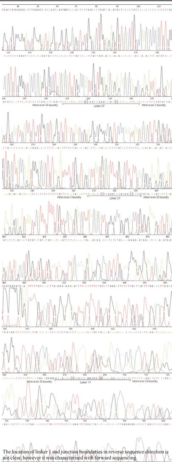
Fig. 6. Sequencing electropherograms from the 850-bp BRCA1 exons 23, 20, 2 and 24 produced by Gene Assembling technique (full-length reverse orientation using primer 10).
