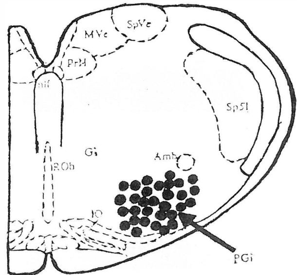
Fig. 3. Reconstruction of a coronal section taken through the rostral medulla showing anatomical maps of recording sites (filled circles) of the PGI neurons in formalin injected rats. Abbreviations: Amb, nucleus ambiguus; Gi, gigantocellular reticular nucleus; IO, inferior olive; MVe, medial vestibular nucleus; mlf, medial longitudinal fasciculus; PGI, paragigantocellular reticular nucleus; PrH, prepositus hypoglossal nucleus; ROb, raphe obscurus nucleus; Sp5I, spinal trigeminal nucleus, interpolar part; SpVe, spinal vestibular nucleus.
