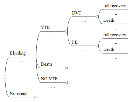
Figure 1. Decision tree
