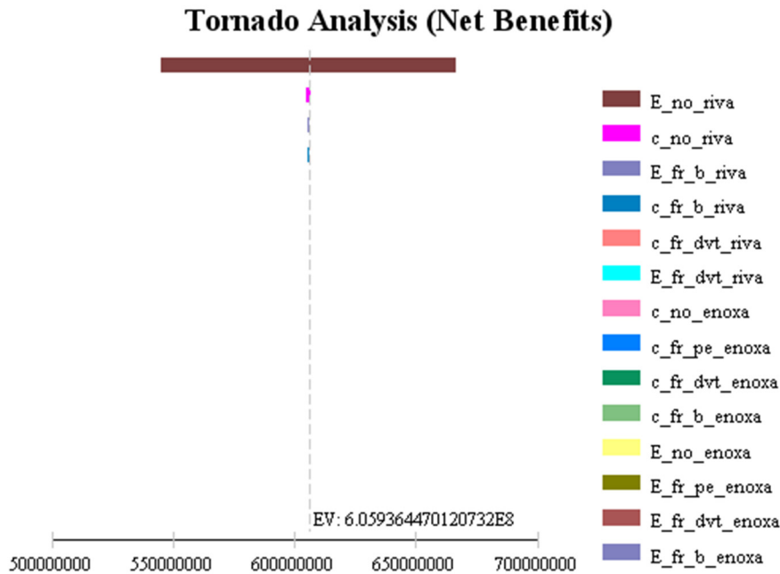
Figure 3. Tornado diagram
