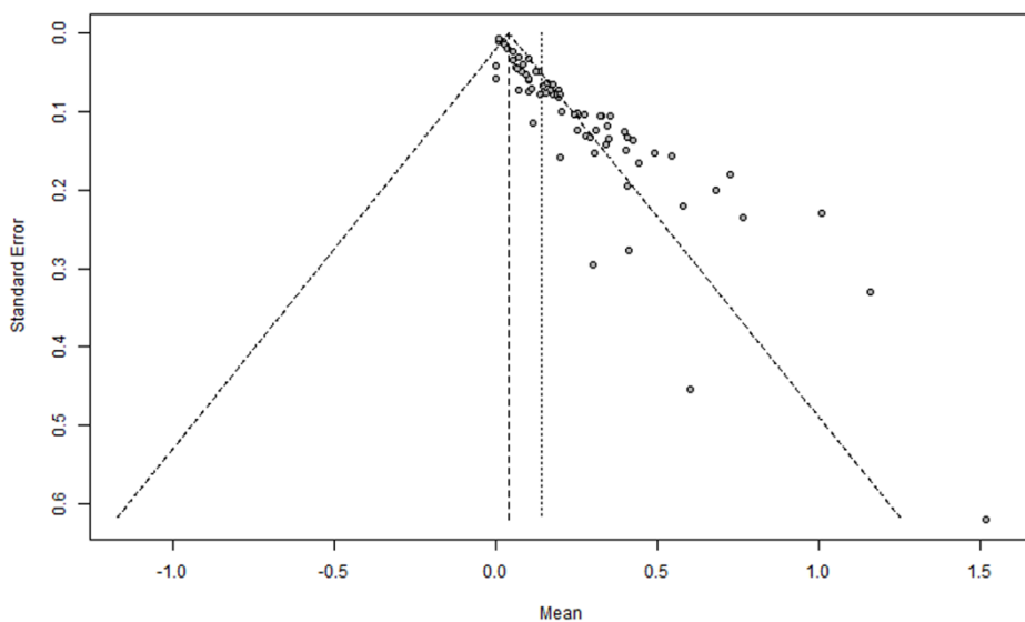
Egger's Test – Test for funnel plot assymetry - F : P < .0001
