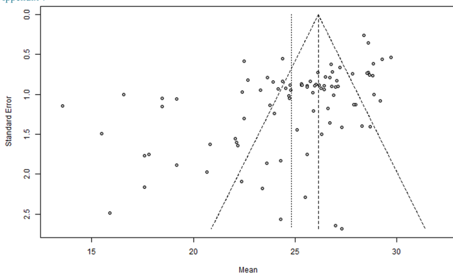
Egger's Test – Test for funnel plot assymetry - M : P < .0001
