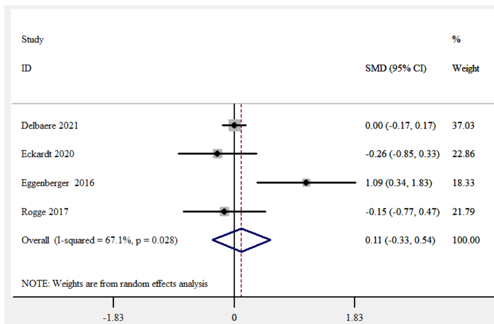
Figure 2. The results of Meta-analysis in Stroop test
