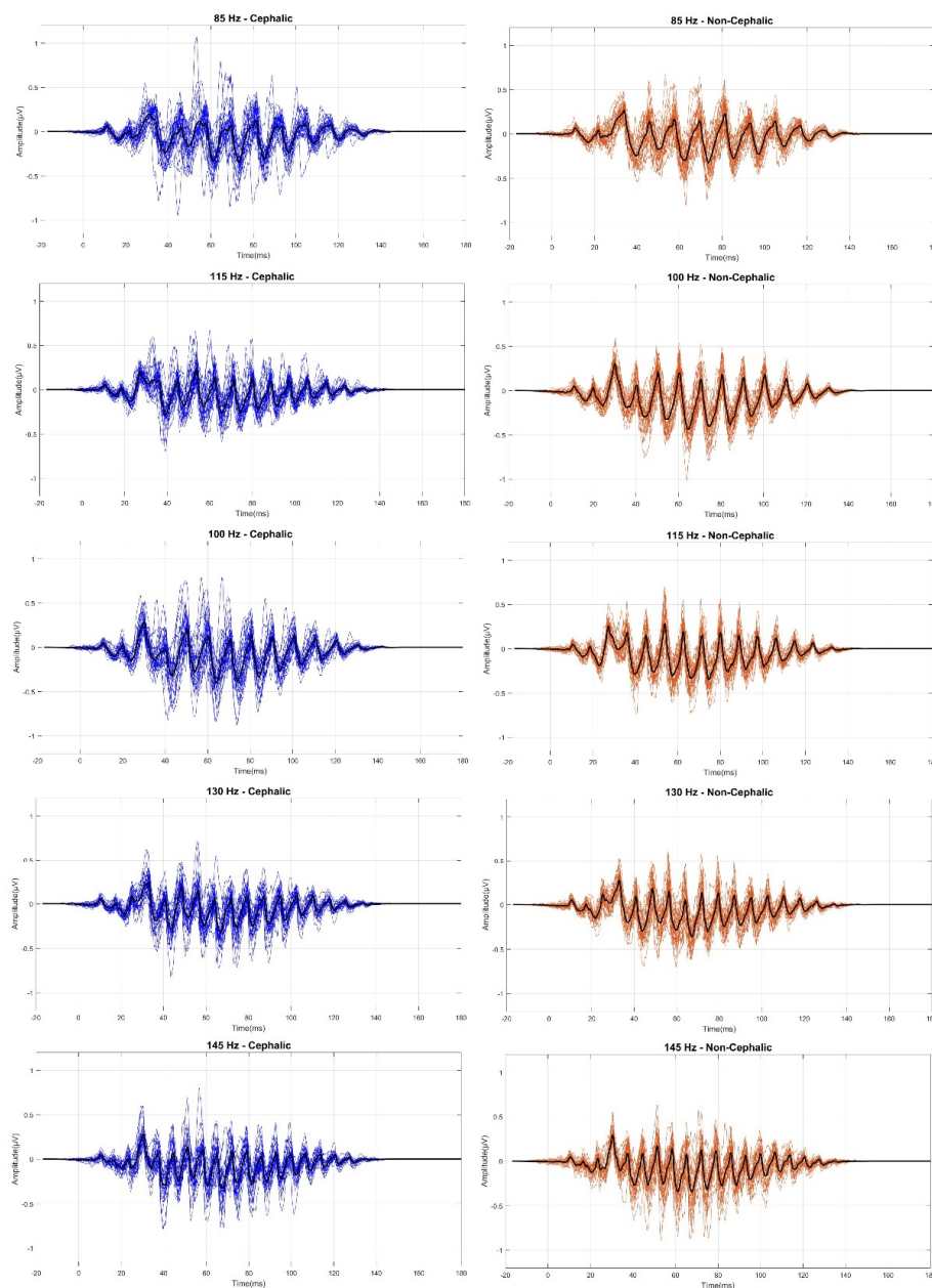
Figure 1. The grand average (thick line) and individual waveforms (thin lines) of FFRs recorded in the cephalic (left column) and non-cephalic(right column) electrode montages in frequencies of 85, 100, 115, 130, and 145 Hz.
